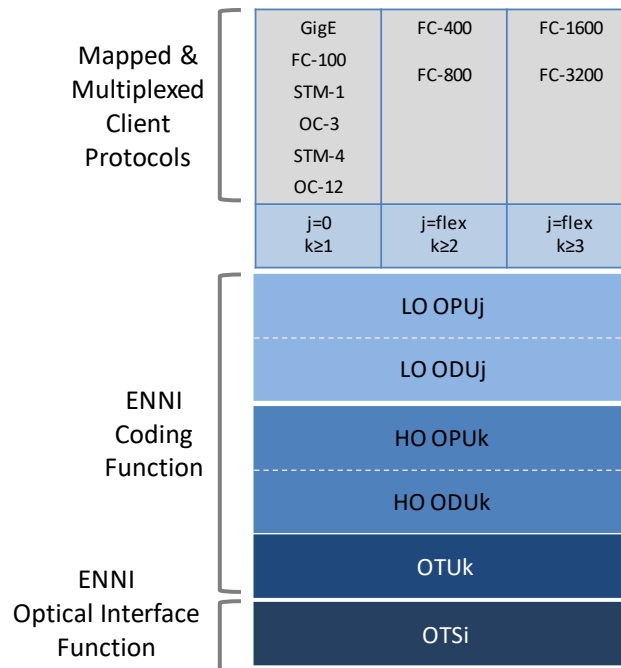
Figure 8 – ENNI Coding & Optical Interface Functions for Mapped & Multiplexed Clients
