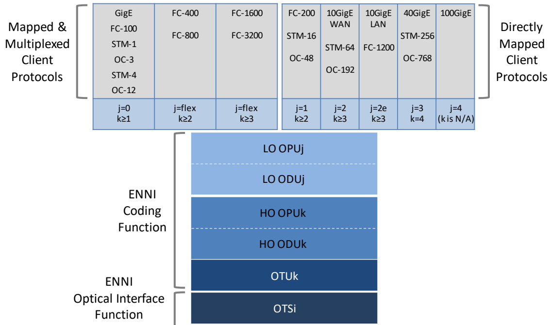
Figure 25 – Example with Directly Mapped Client Protocols included in HO Multiplexing
