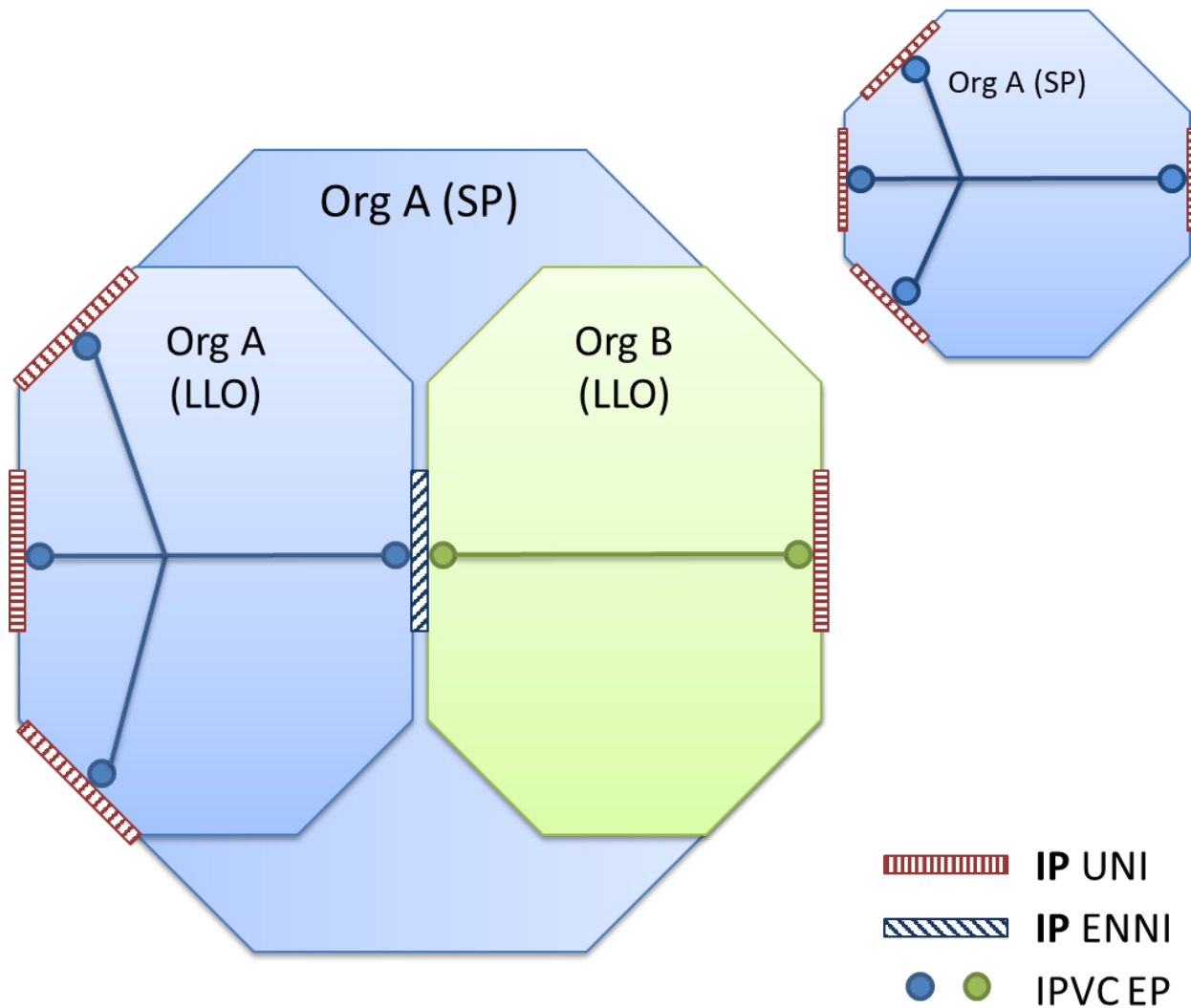
Figure 65 – Access to a Single Remote UNI
