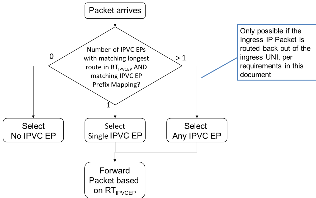
Figure 24 – Selecting an Ingress IPVC EP
