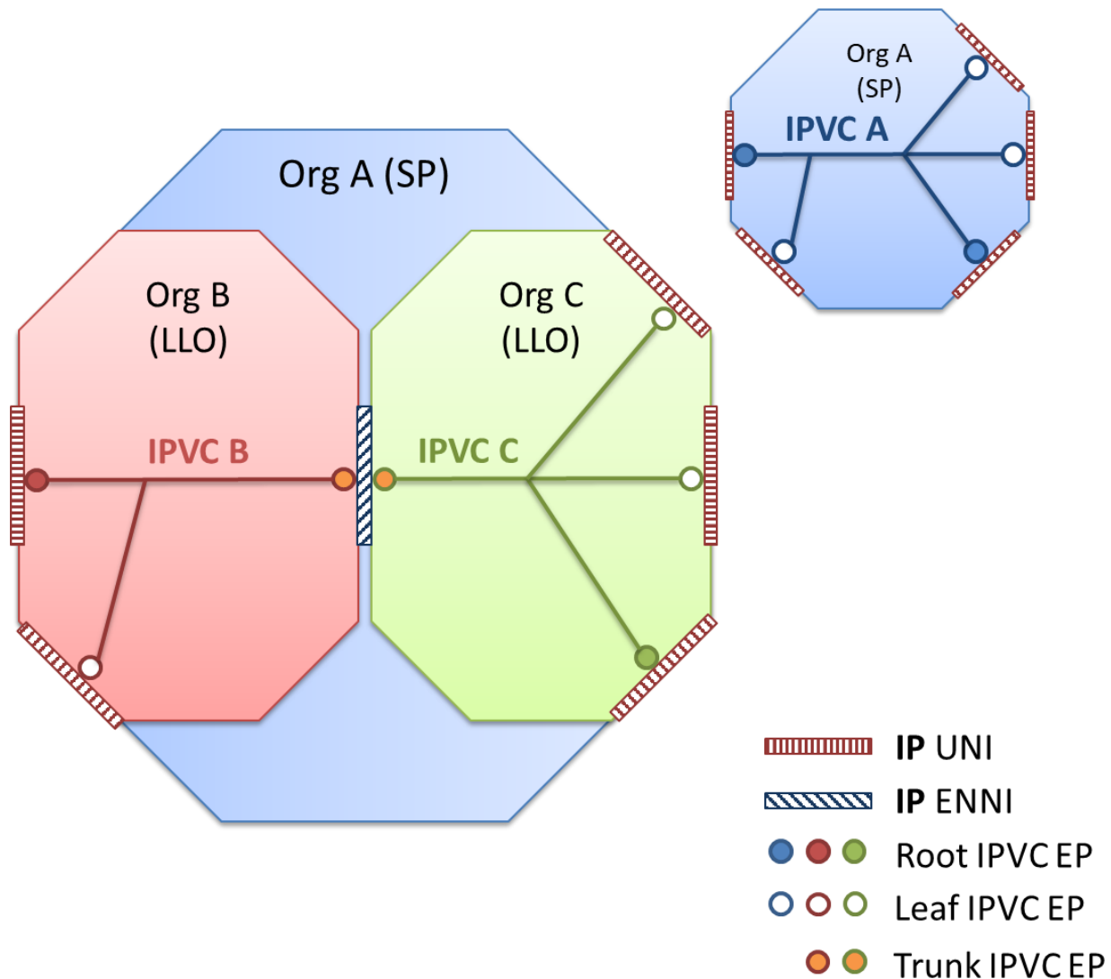
Figure 20 – Example of a Rooted Multipoint IPVC across an ENNI with Trunk IPVC EPs
