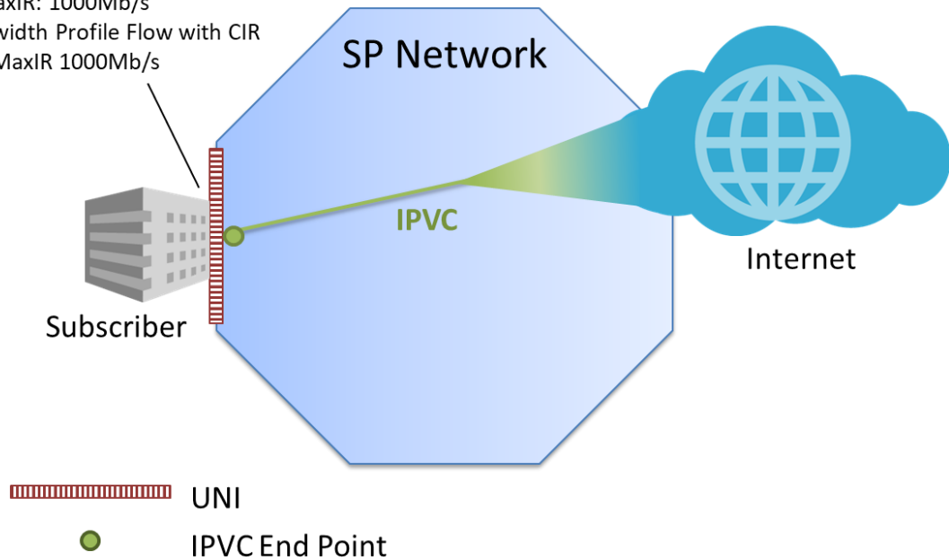
Figure 55 – Bandwidth Profile Example for an Internet Access Service
