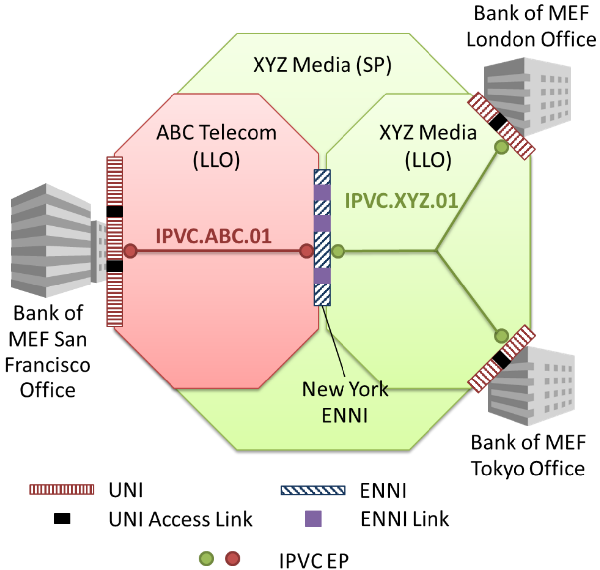
Figure 77 – Example Operator Services used for a Multipoint IP VPN
