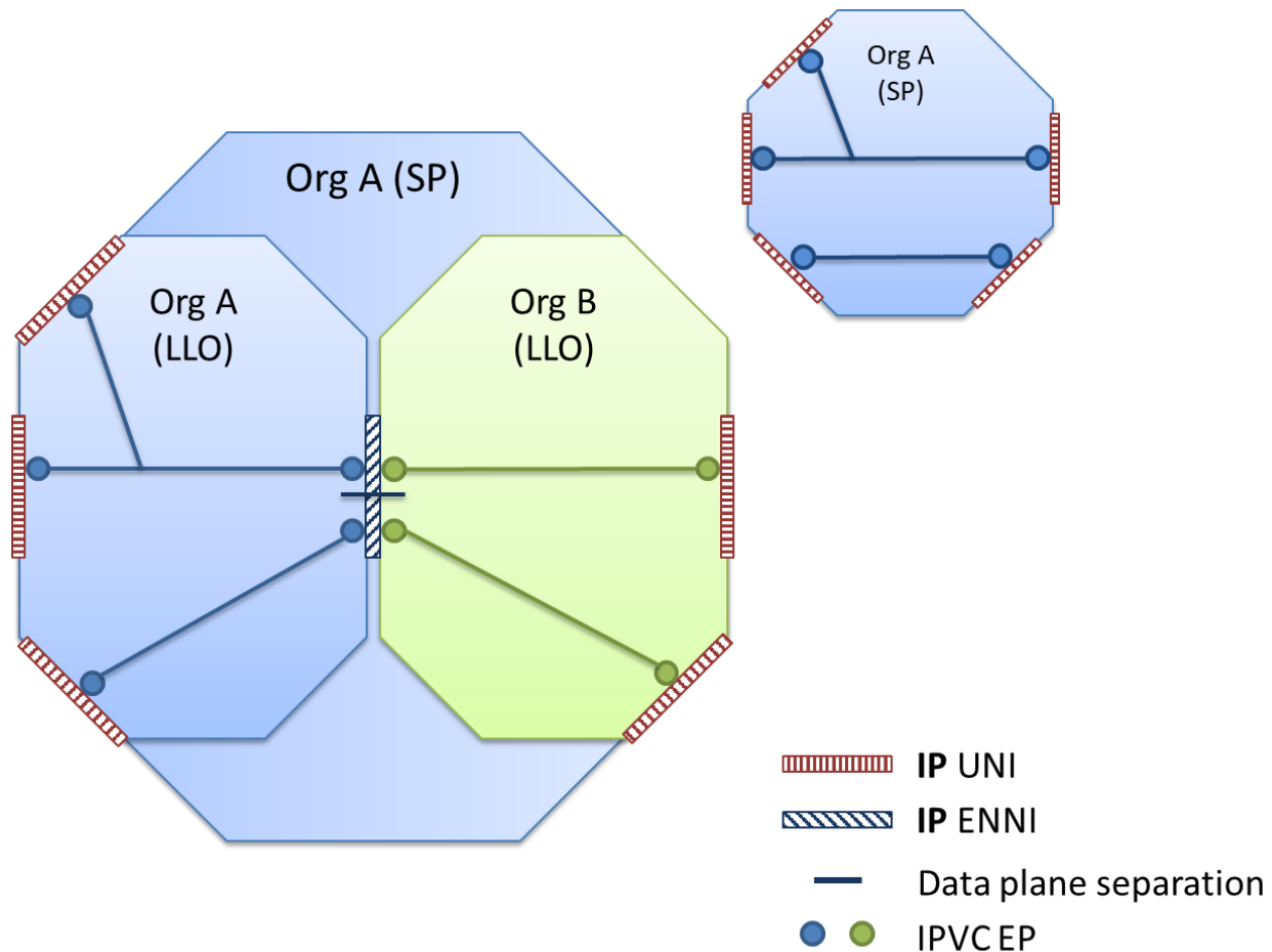
Figure 67 – Multiple Services at an ENNI
