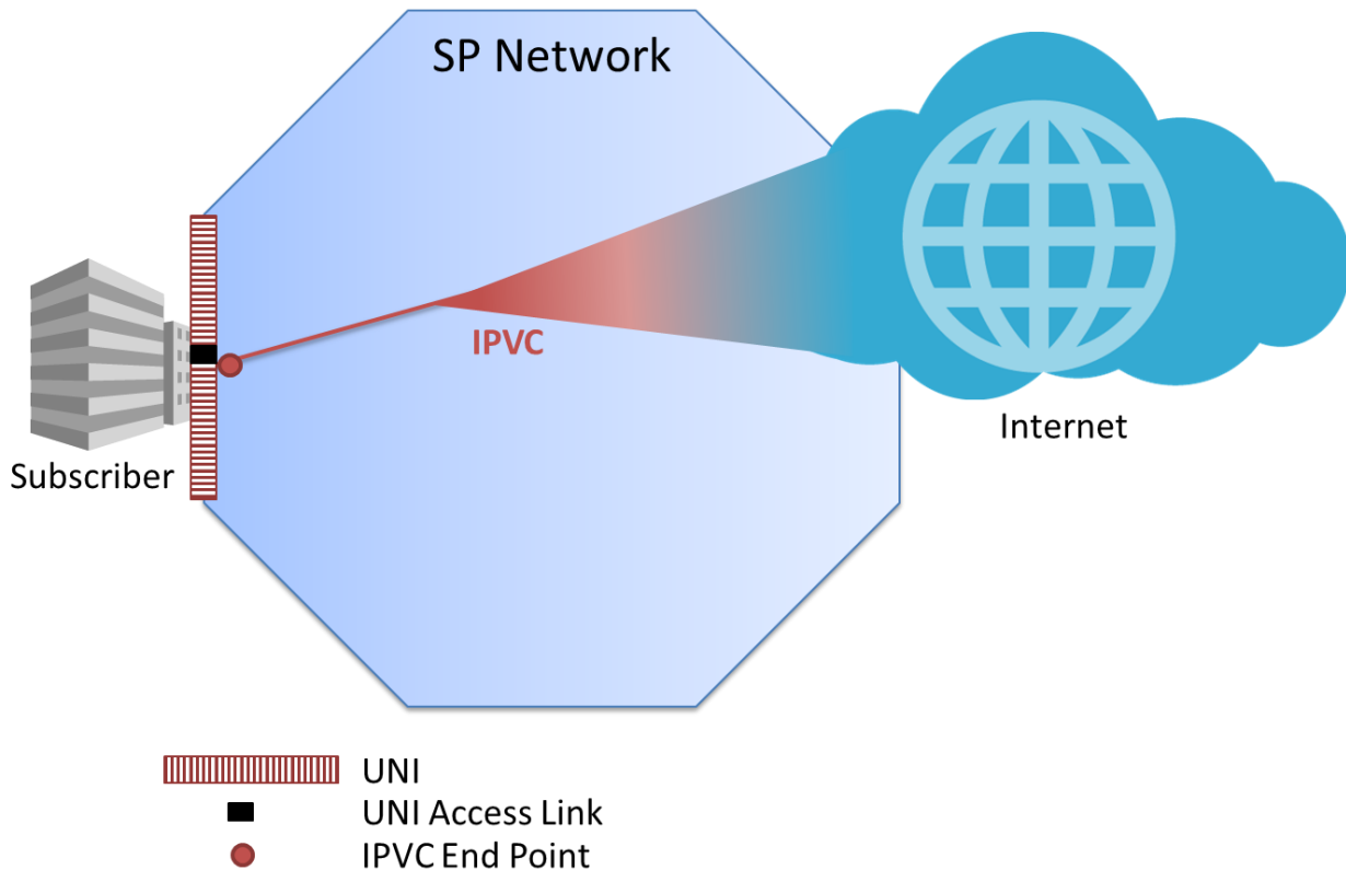
Figure 64 – Example Cloud Access IPVC for Internet Access
