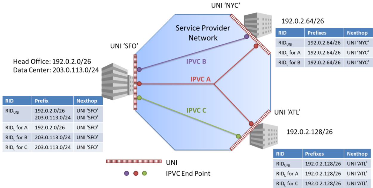
Figure 37 – Example IP Service – Reachable Prefixes
