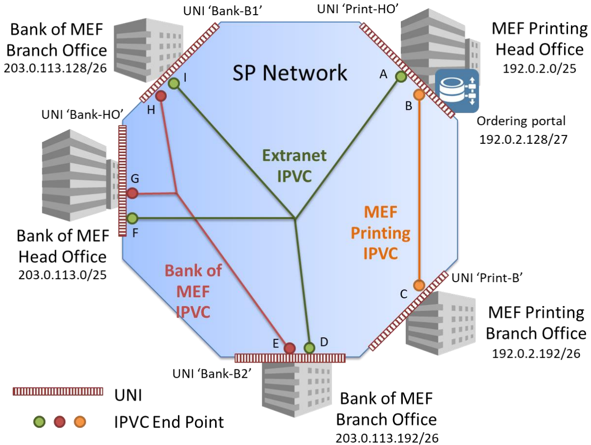
Figure 41 – Extranet Example showing IP Prefixes
