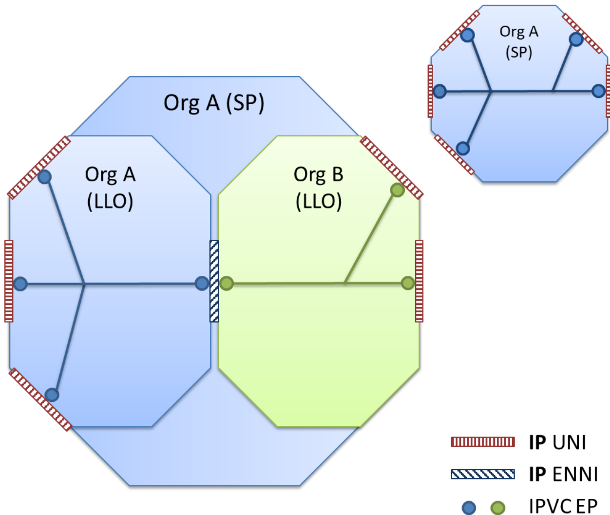
Figure 66 – Access to Multiple Remote UNIs
