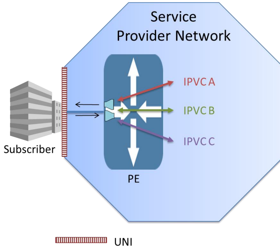
Figure 59 – Example per-UNI Traffic Conditioning Location for Multiple IPVCs
