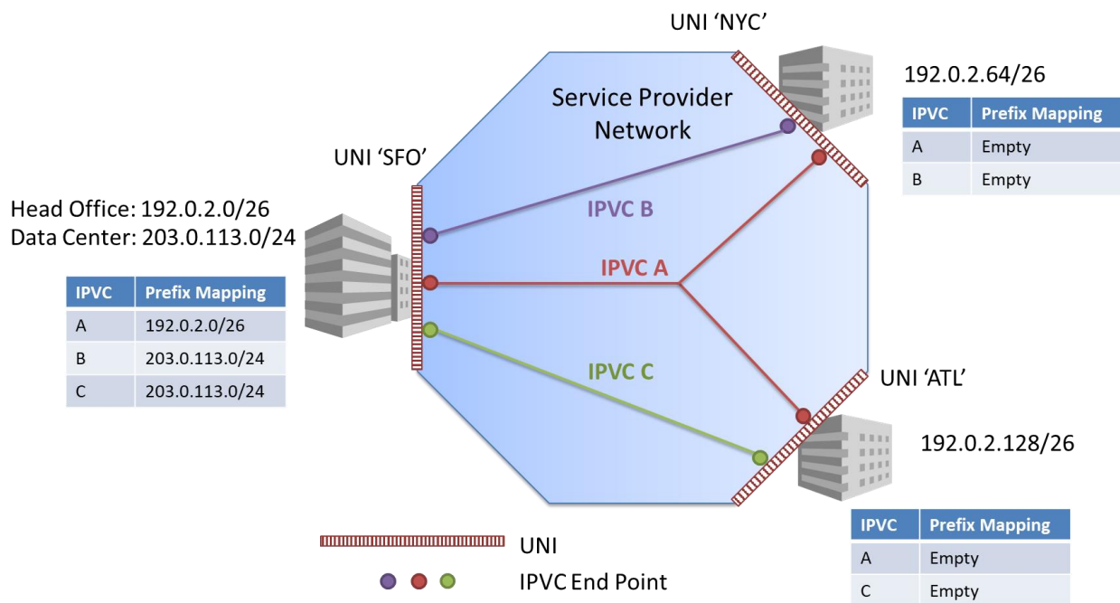
Figure 36 – Example IP Service – Subnets and Prefix Mapping
