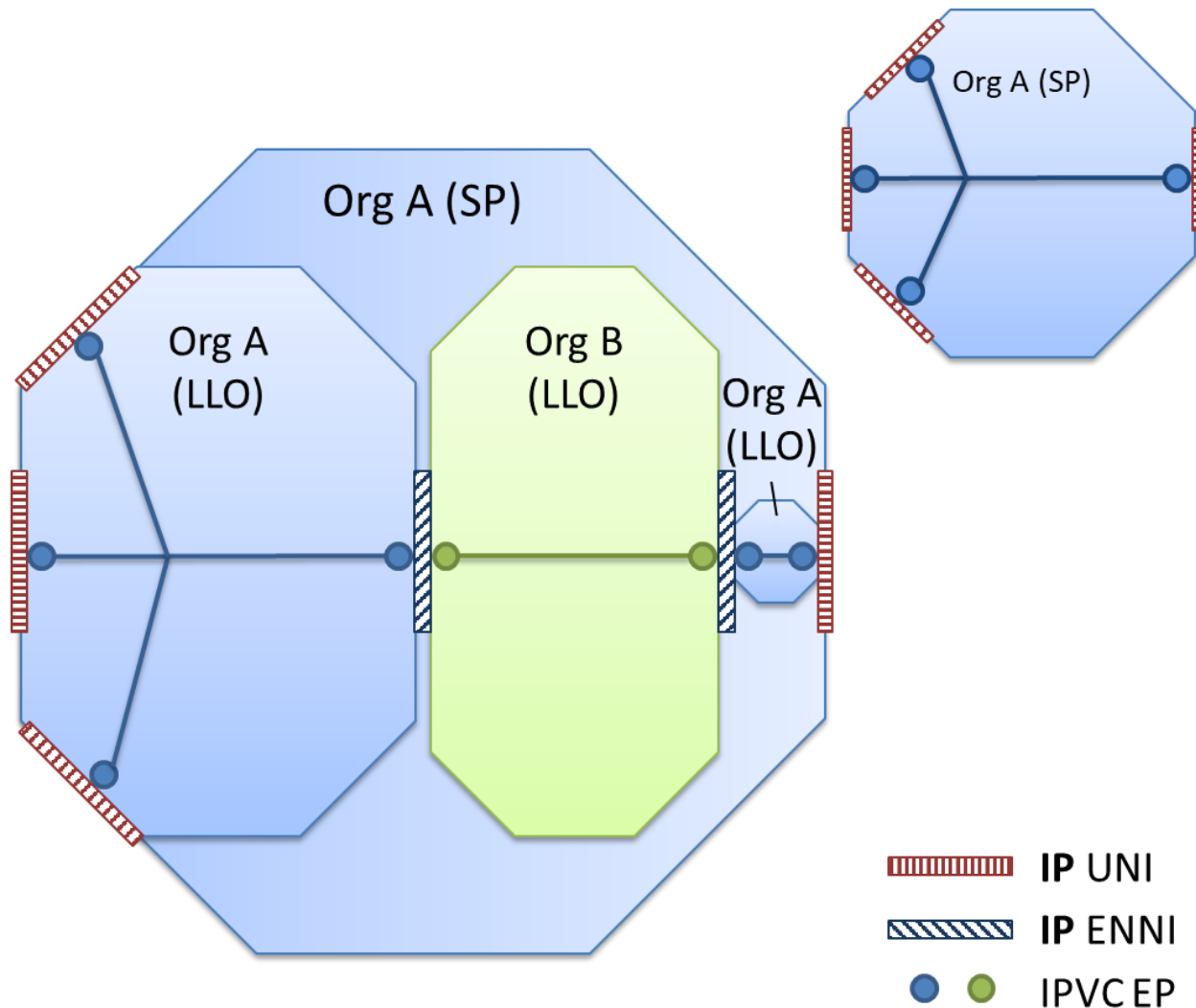
Figure 69 – Operator Transit Service Connecting an SP Managed CPE
