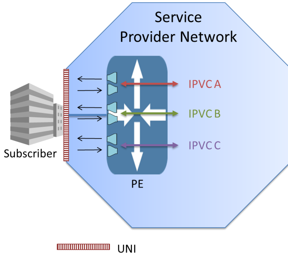
Figure 58 – Example per-IPVC Traffic Conditioning Location for Multiple IPVCs
