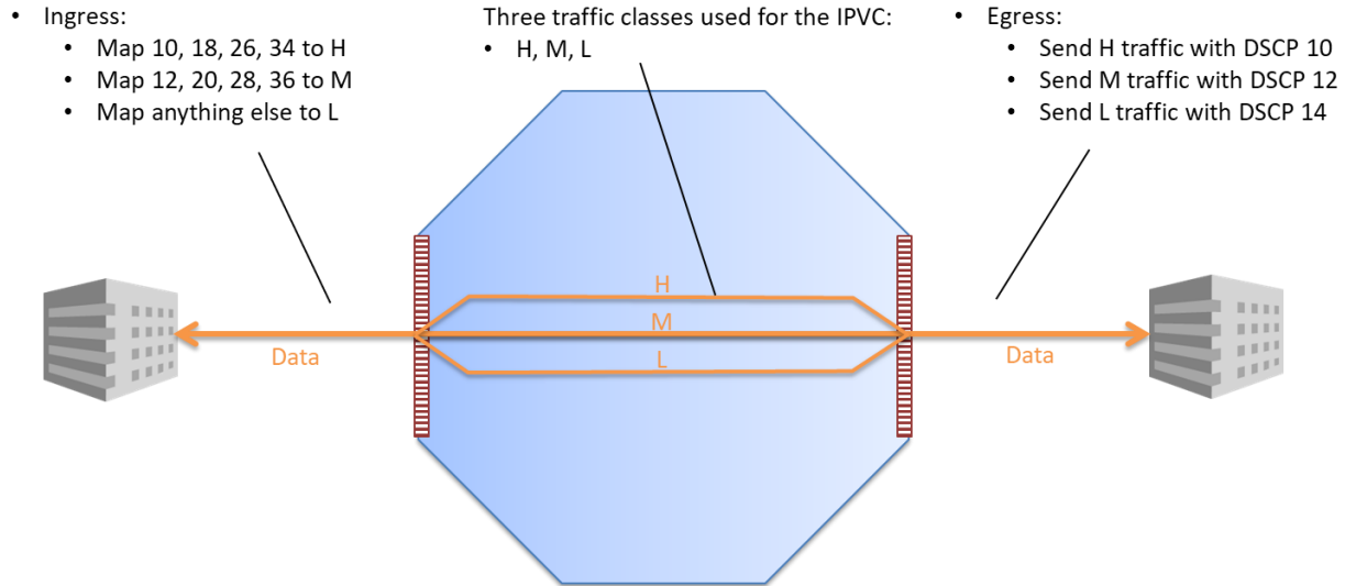
Figure 49 – Example of an Egress CoS Map
