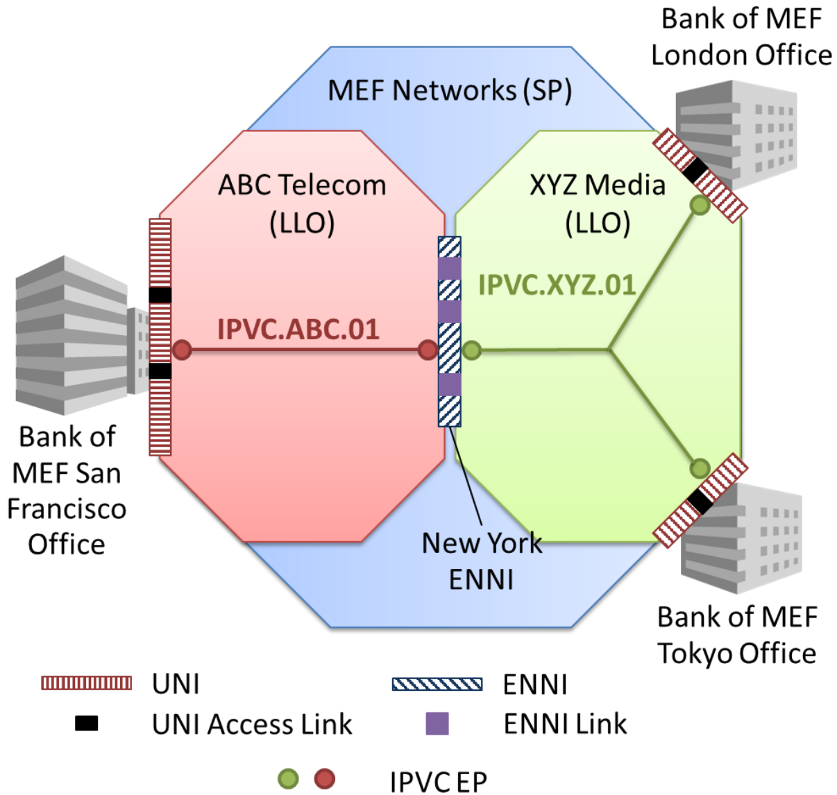
Figure 76 – Example Operator Services used for a Multipoint IP VPN
