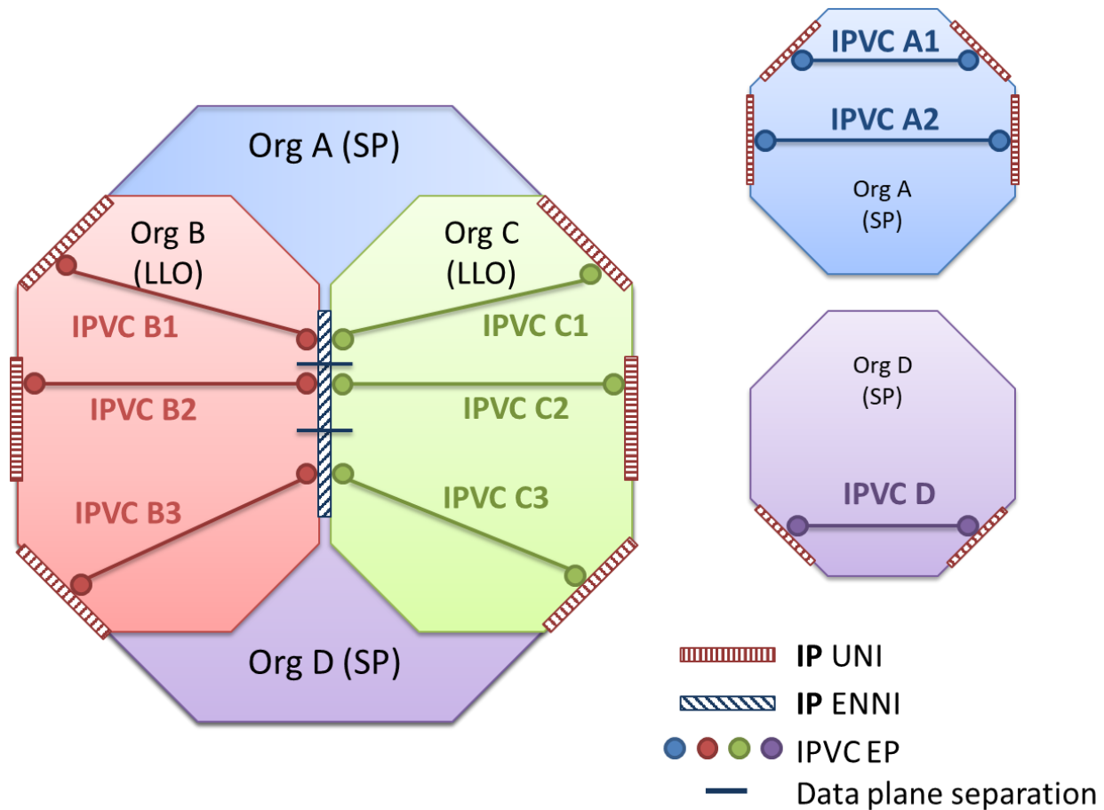
Figure 30 – Example for ENNI Service Map
