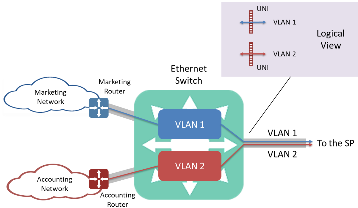
Figure 33 – Example of Multiple Subscriber Networks – Setup at one Location
