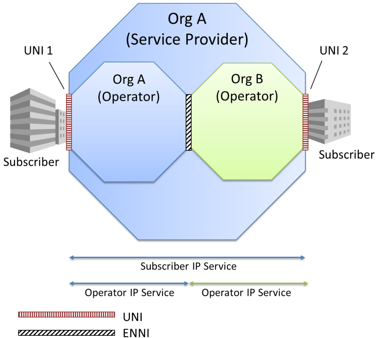
Figure 14 – Operator IP Services with the SP acting as an Operator
