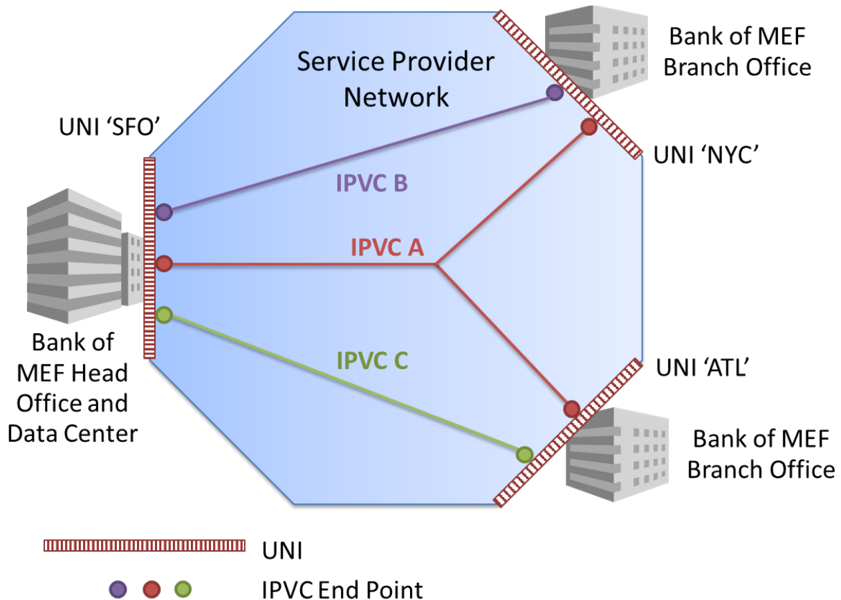
Figure 35 – Example IP Service Showing Three IPVCs
