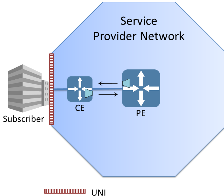
Figure 60 – Example Traffic Conditioning Location for a Provider-Managed CE
