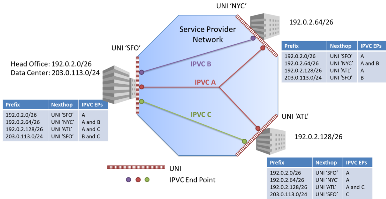
Figure 39 – Example IP Service – Combined Routing
