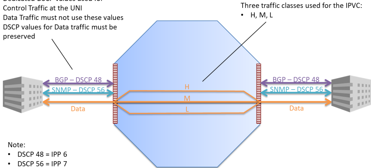
Figure 46 – Example with DSCP Preservation
