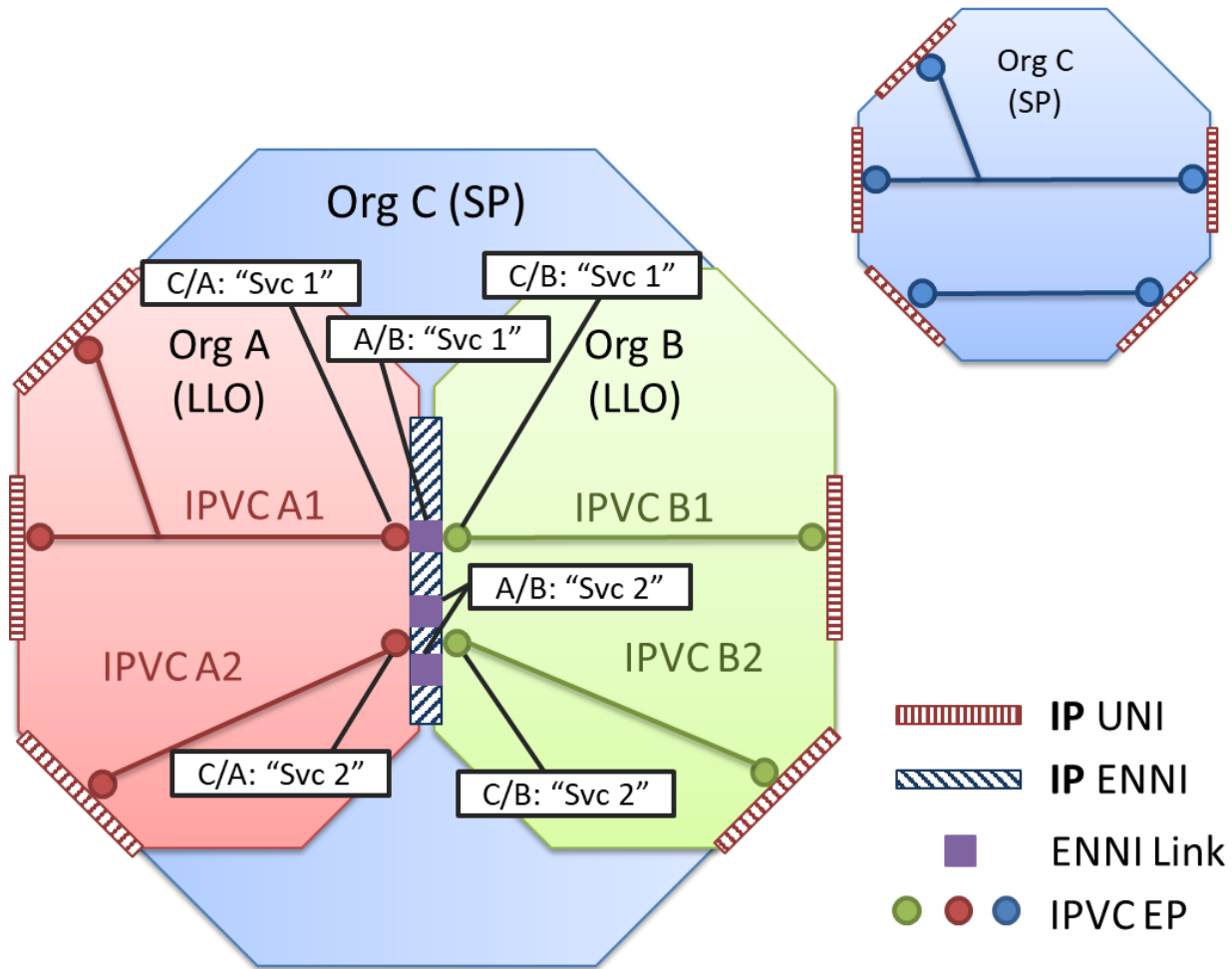
Figure 18 – Example of ENNI Service Mapping Identifiers for IP Services across an ENNI
