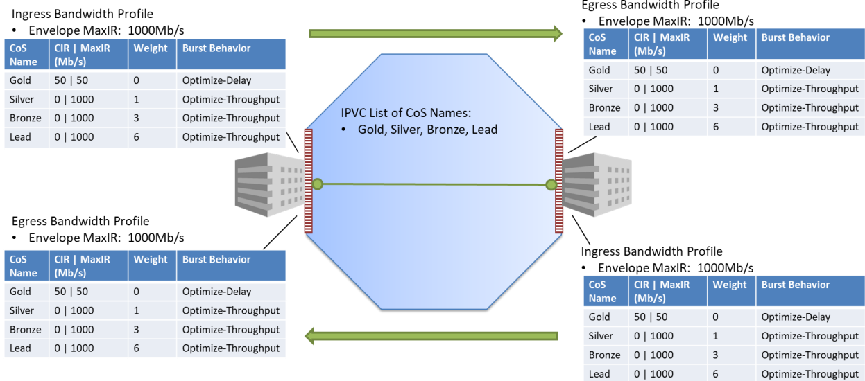
Figure 54 – Bandwidth Profile Example for an IP VPN Service
