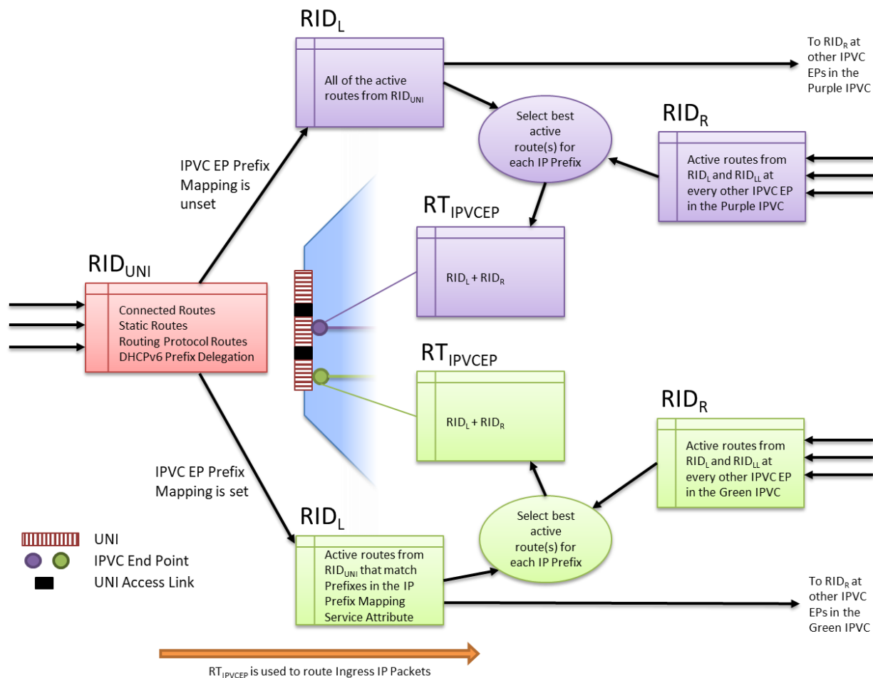
Figure 21 – Routing Information Databases at a UNI (IPVC EPs with Root role)
