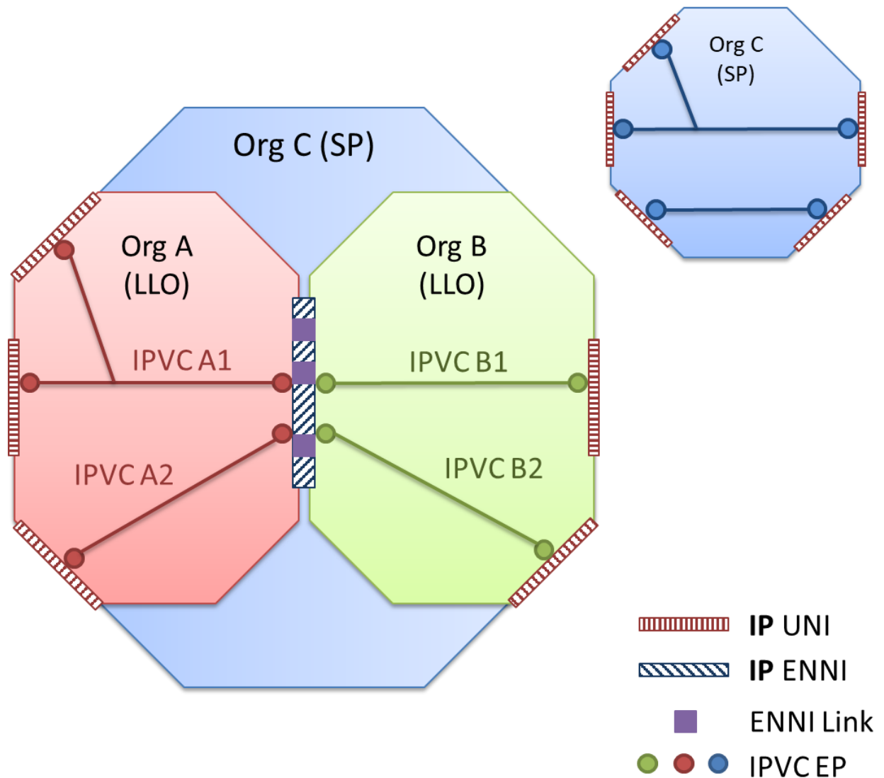
Figure 17 – Example of two IP Services across and ENNI
