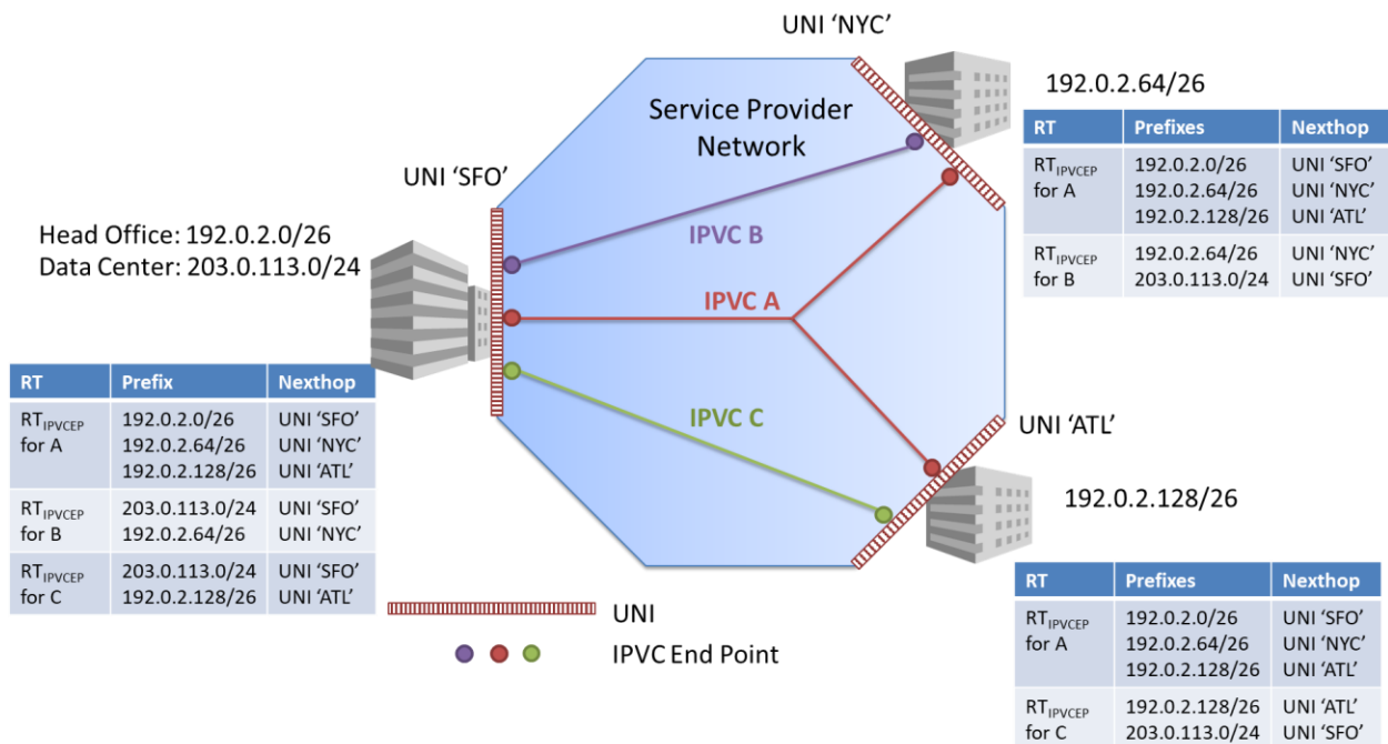
Figure 38 – Example IP Service – Per-IPVC EP Routing
