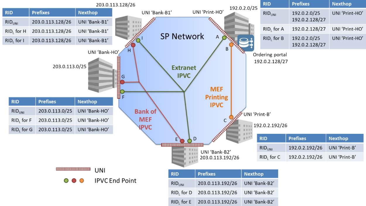
Figure 42 – Extranet Example showing Routing Information Databases
