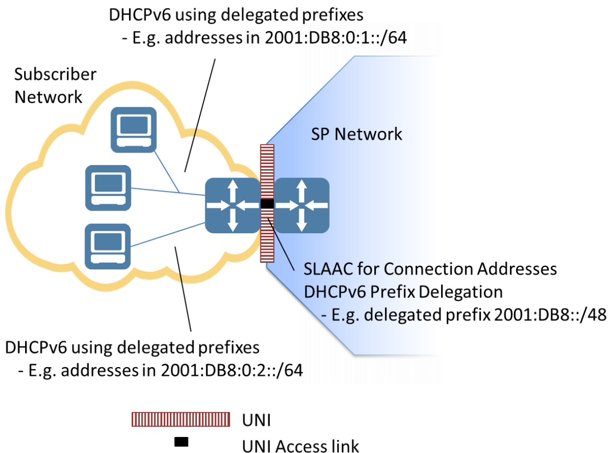
Figure 29 – DHCPv6 Prefix Delegation
