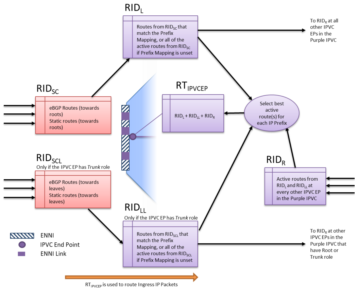
Figure 22 – Routing Information Databases at an ENNI
