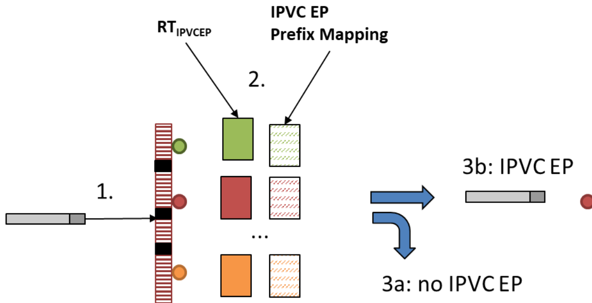
Figure 23 – IP Packet Delivery overview
