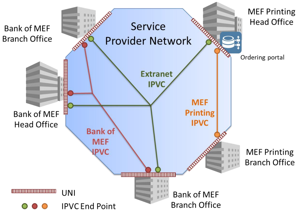
Figure 40 – Extranet Example showing IPVCs
