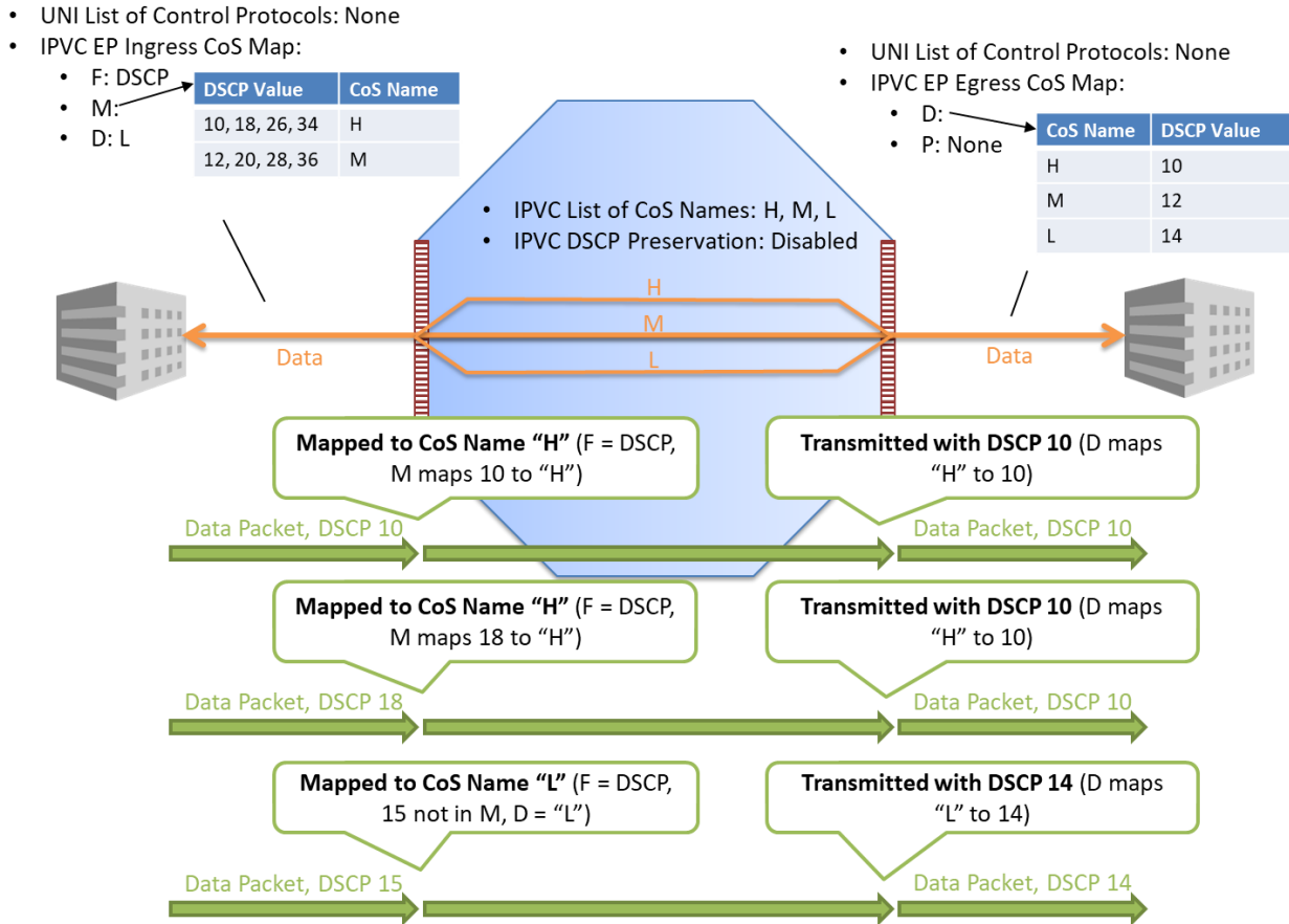
Figure 51 – Example of an Egress CoS Map showing packet handling
