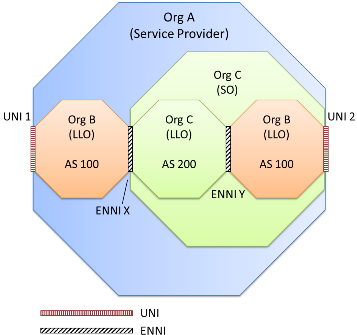
Figure 70 – Example of AS Override at an ENNI
