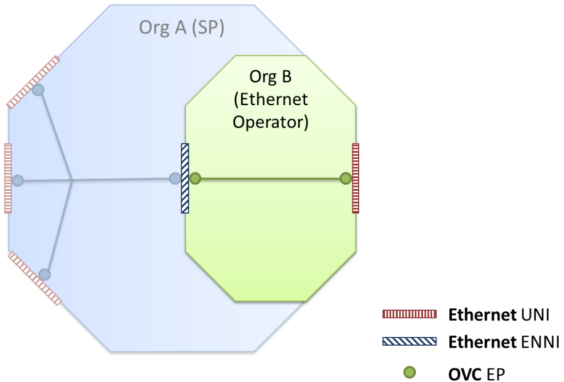
Figure 73 – Access E-Line connecting to an IP Service.
