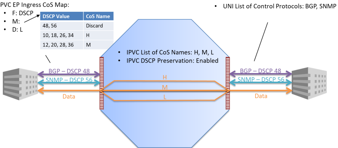
Figure 47 – Example with DSCP Preservation showing Service Attributes
