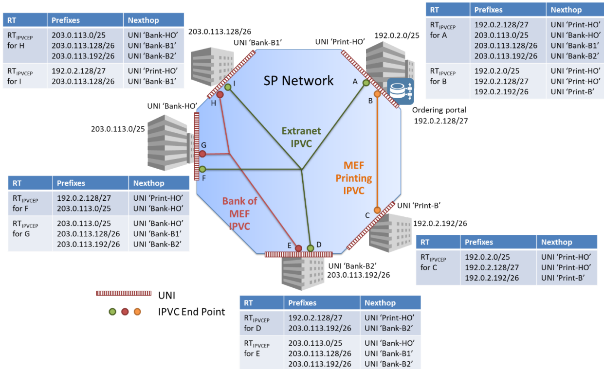
Figure 43 – Extranet Example showing Routing Tables
