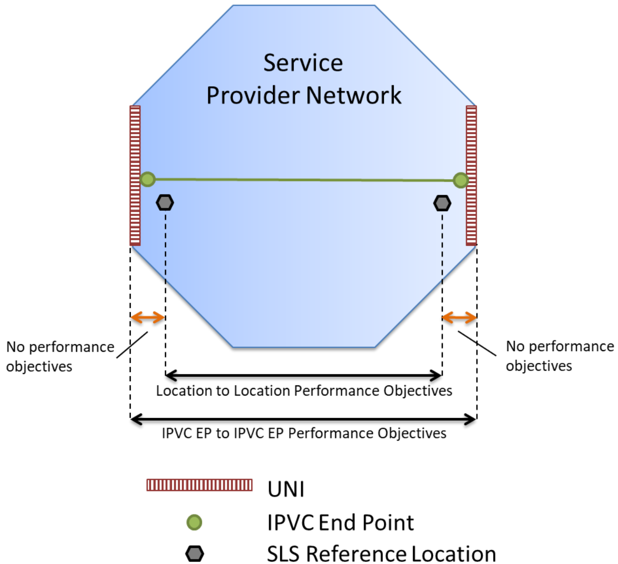
Figure 26 – Example of SLS specified using locations
