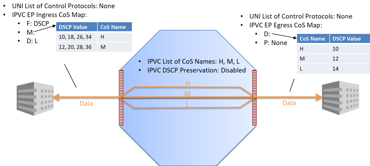
Figure 50 – Example of an Egress CoS Map showing Service Attributes
