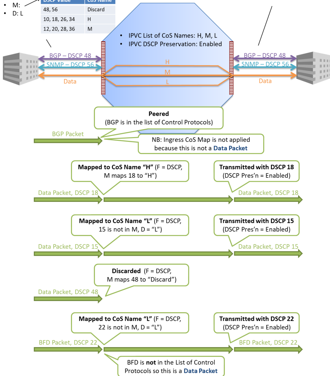
Figure 48 – Example with DSCP Preservation showing packet handling
