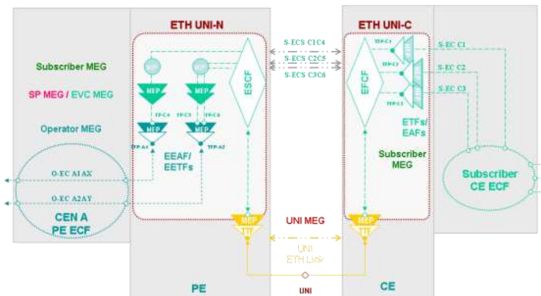
Figure 3 – MEP Placement
