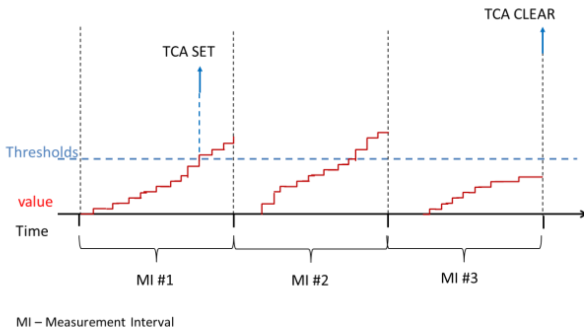
Figure 15 – Stateful TCA Reporting Example
