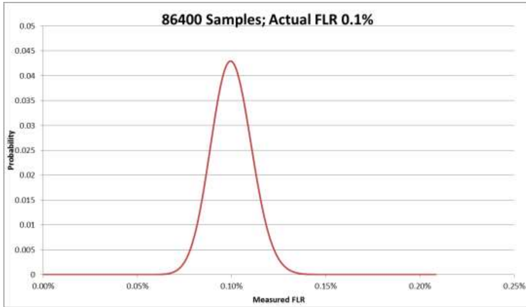
Figure 33 – Synthetic Loss Performance Example 3
