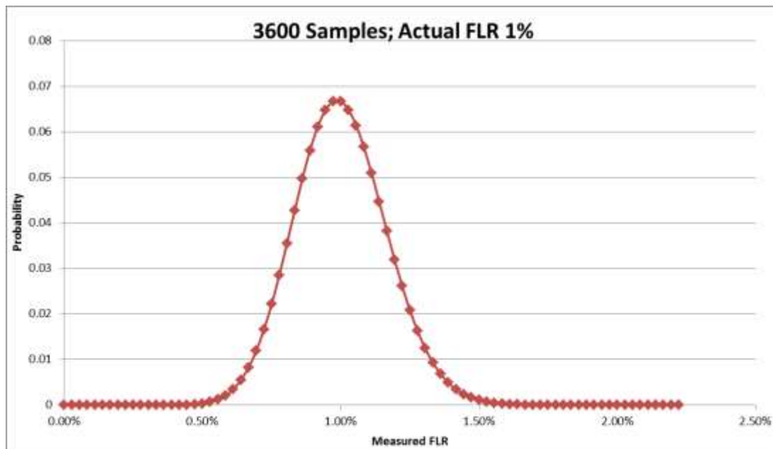
Figure 31 – Synthetic Loss Performance Example 1
