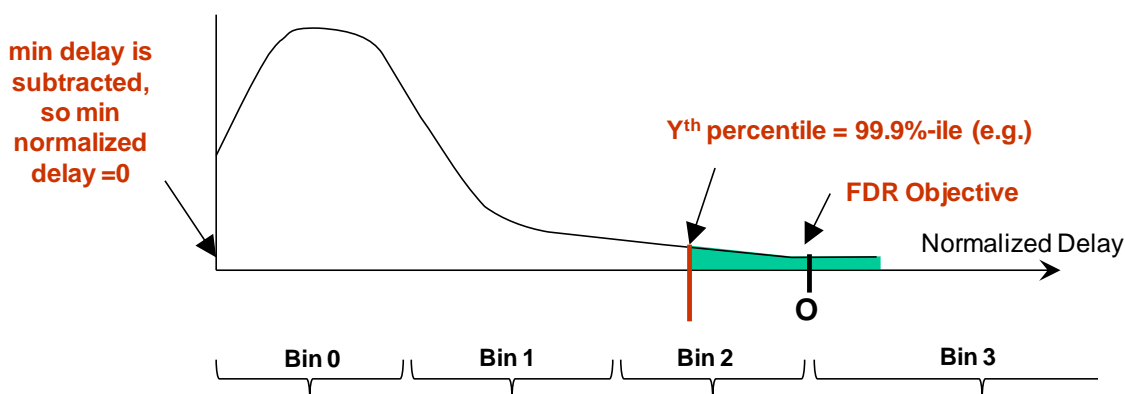
Figure 36 – Example FDR Distribution (normalized), and Bins
