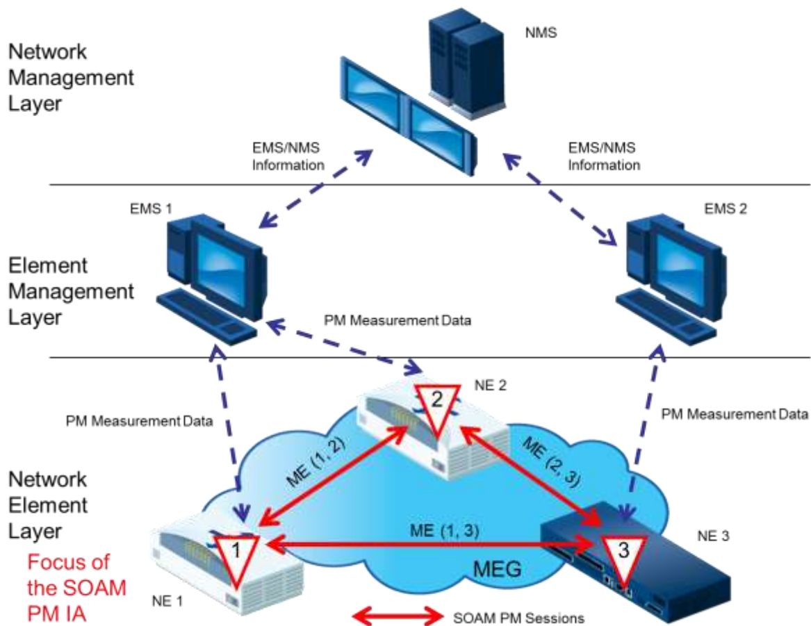
Figure 7 – PM Solution Components
