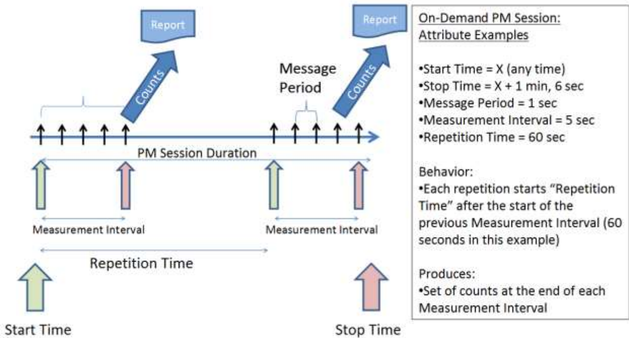
Figure 25 – Example of Repetitive On-Demand PM Session
