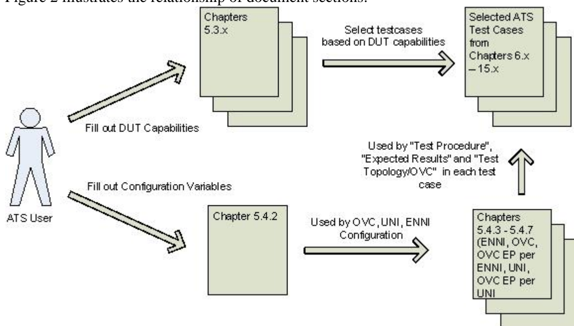
Figure 2: ATS Structure
