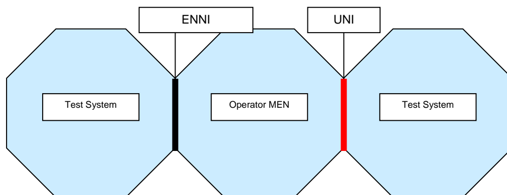
Figure 3: Test Topology 1
