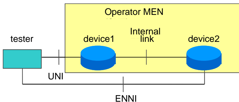
Figure 9: Multiple device MEN
