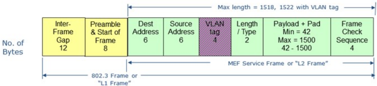
Figure 6. Length of an Ethernet frame as measured with and without the 20 byte inter-frame overhead.
