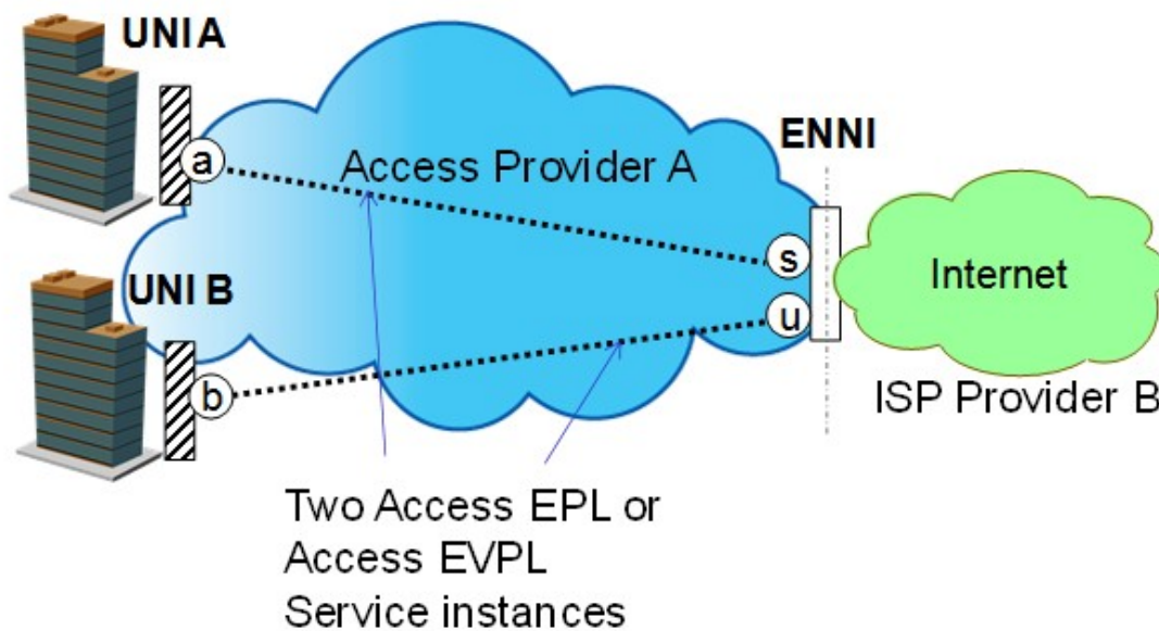
Figure 12. Access aggregation to Layer 3 services using Access EPL or Access EVPL.
