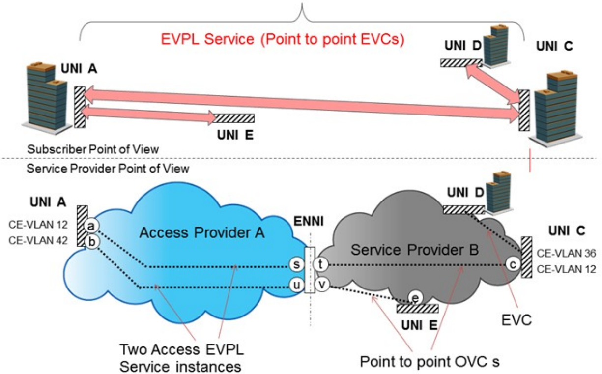
Figure 11. EVPL Service as implemented across two networks using Access EVPL, showing the Subscriber and Service Provider POVs.
