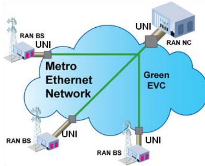
Figure 14: Ethernet Private Tree (EP-Tree) Service
