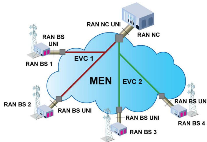
Figure 25: EVP-Tree per group of RAN BSs – Use Case 2
