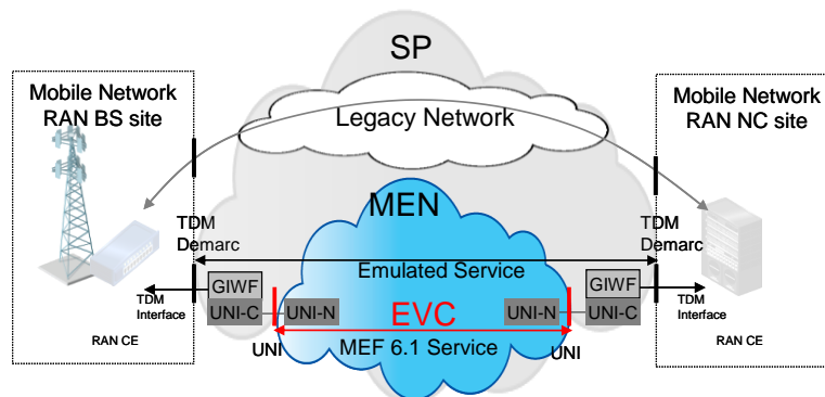
Figure 5: Use Case 1a – Low Priority traffic using CES across MEN
