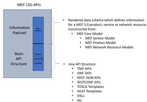
Figure 2: LSO Sonata API Base and Payload
